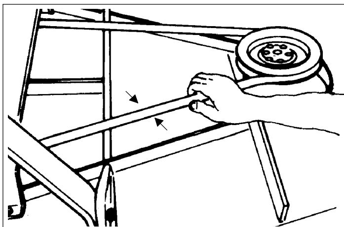
Fig. 12 The belt deflection should be between 8-10 mm. ( \frac{5}{16} "- \frac{3}{8} ").
