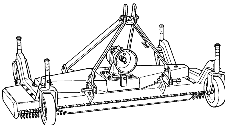
Fig. 3 Rear discharge C50 mower, front mounted.
