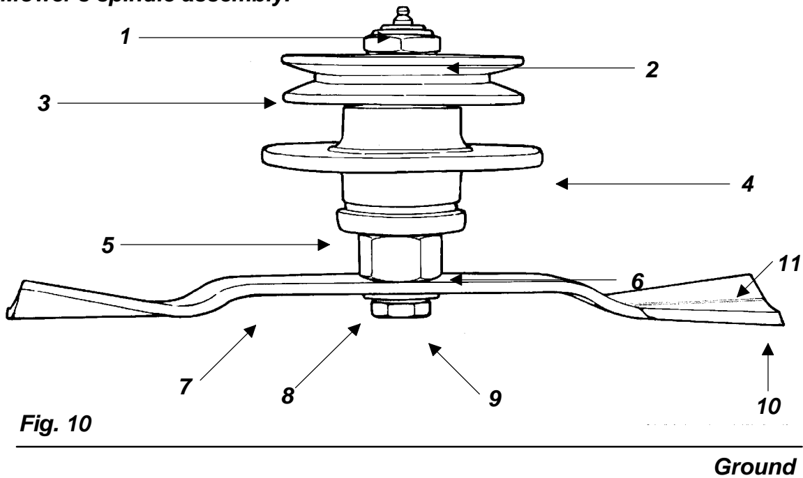
Mower's spindle assembly.
